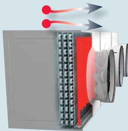
Defrosting without the FabricAir® DefrostDuct™
