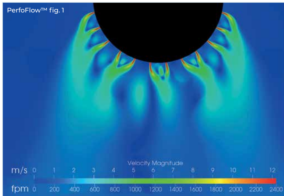
Air discharge through PerfoFlow™ perforation at 120 Pa [ \approx 0.5 iwg].
